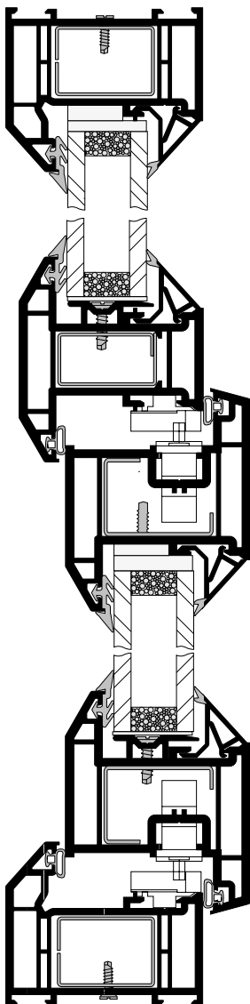
General assembly, internally glazed
